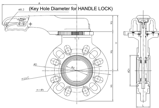
[LEVER TYPE]
